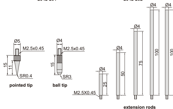
extension rods
