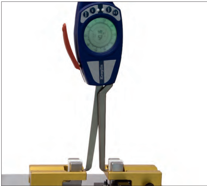
KIT A300005 for inside micrometer heads, Interapid, Kroeplin.
